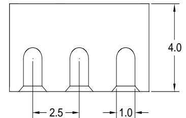
TYPE B (CLOSE END)
