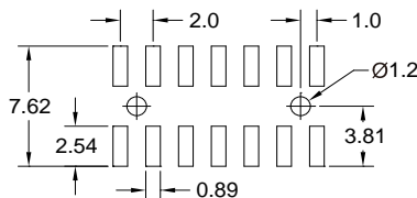
(TYPE A) RECOMMENDED.P.C.B.LAYOUT
