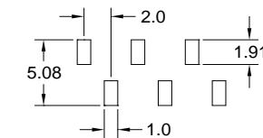
(TYPE B1) RECOMMENDED.P.C.B.LAYOUT
