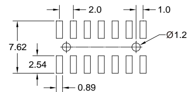
RECOMMENDED.P.C.B.LAYOUT
