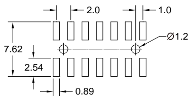
RECOMMENDED.P.C.B.LAYOUT
