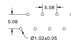
TYPE B2 RECOMMENDED P.C.B LAYOUT
