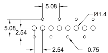
TYPE B2 RECOMMENDED P.C.B LAYOUT
