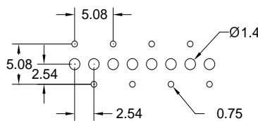
TYPE B1 RECOMMENDED P.C.B LAYOUT
