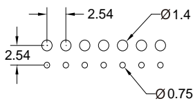
TYPE A RECOMMENDED P.C.B LAYOUT
