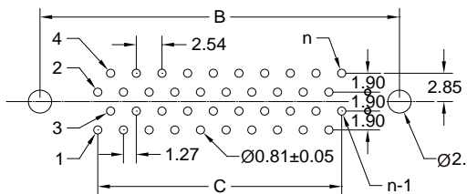
P.C. BOARD LAYOUT FOR 16,20,32,40,60,68,80,100
