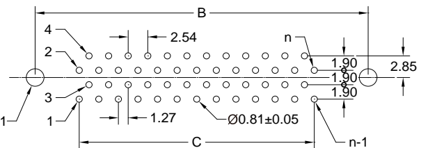
P.C. BOARD LAYOUT FOR 10,14,26,30,34,50
