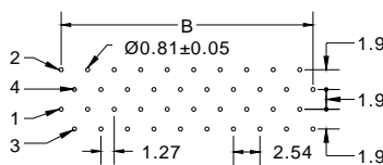
P.C. BOARD LAYOUT FOR 20,40,60,68,80,100
