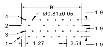
P.C. BOARD LAYOUT FOR 10,26,30,34,50,70,90
