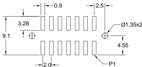
RECOMMENDED.P.C.B.LAYOUT
