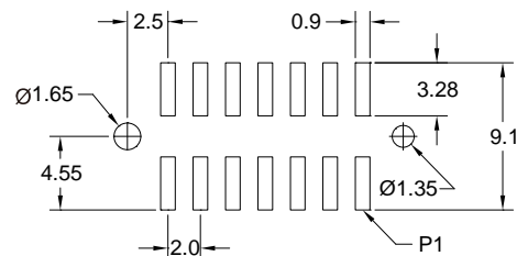
RECOMMENDED.P.C.B.LAYOUT
