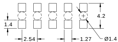
RECOMMENDED DUAL ENTRY P.C.B LAYOUT
